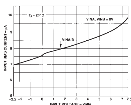
Figure 18. Input Bias Current vs. Input Voltage
