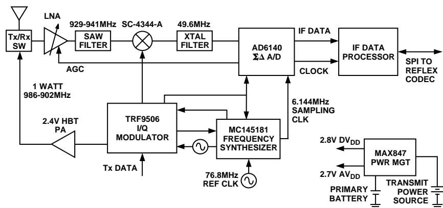
Figure 11. ReFLEX Transceiver Block Diagram
