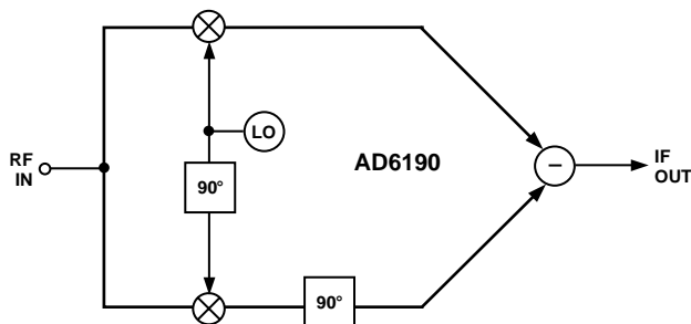
Figure 9. Image-Reject Mixer
