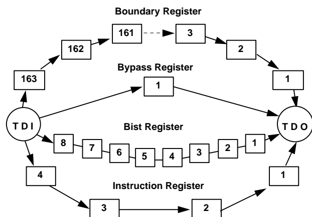
Figure 10. JTAG Registers
