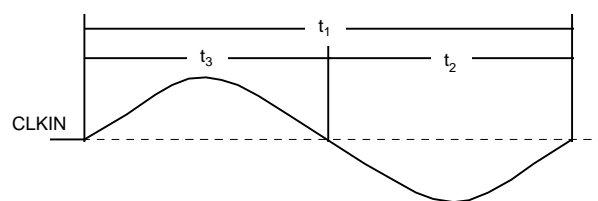
Figure 13. Clock Input
