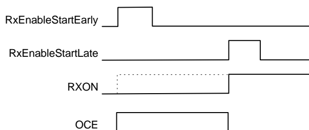
Figure 9. OCE Signal
