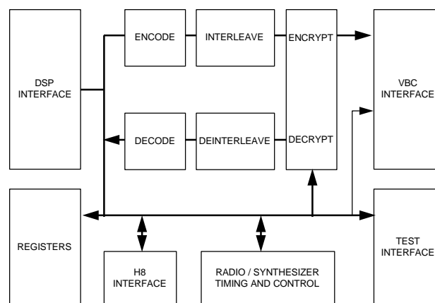
Figure 3. Channel Codec Subsystem
