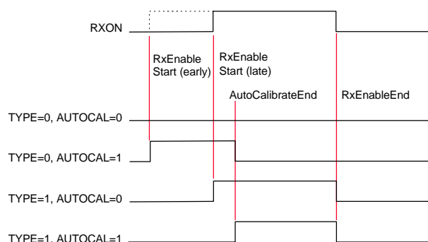
Figure 8. Autocalibration
