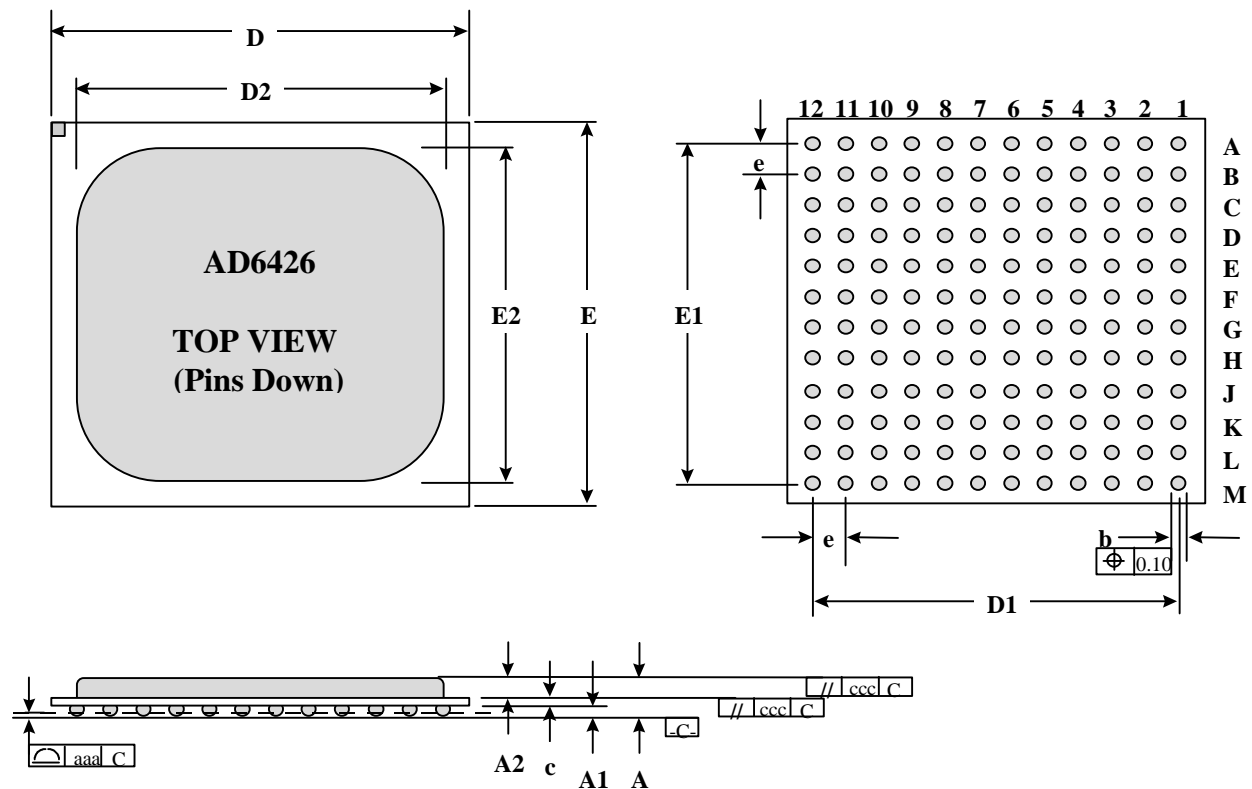
PBGA Outline Dimensions
