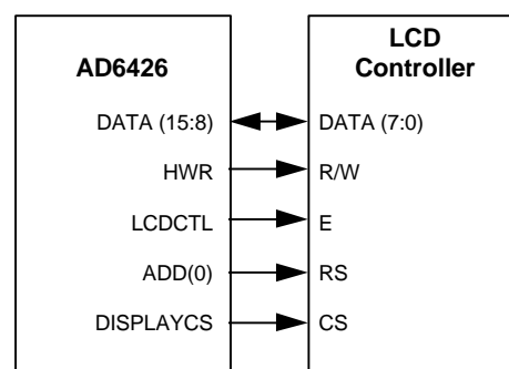
Figure 5. Parallel Display Interface
