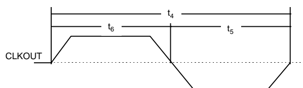
Figure 14. Clock Output
