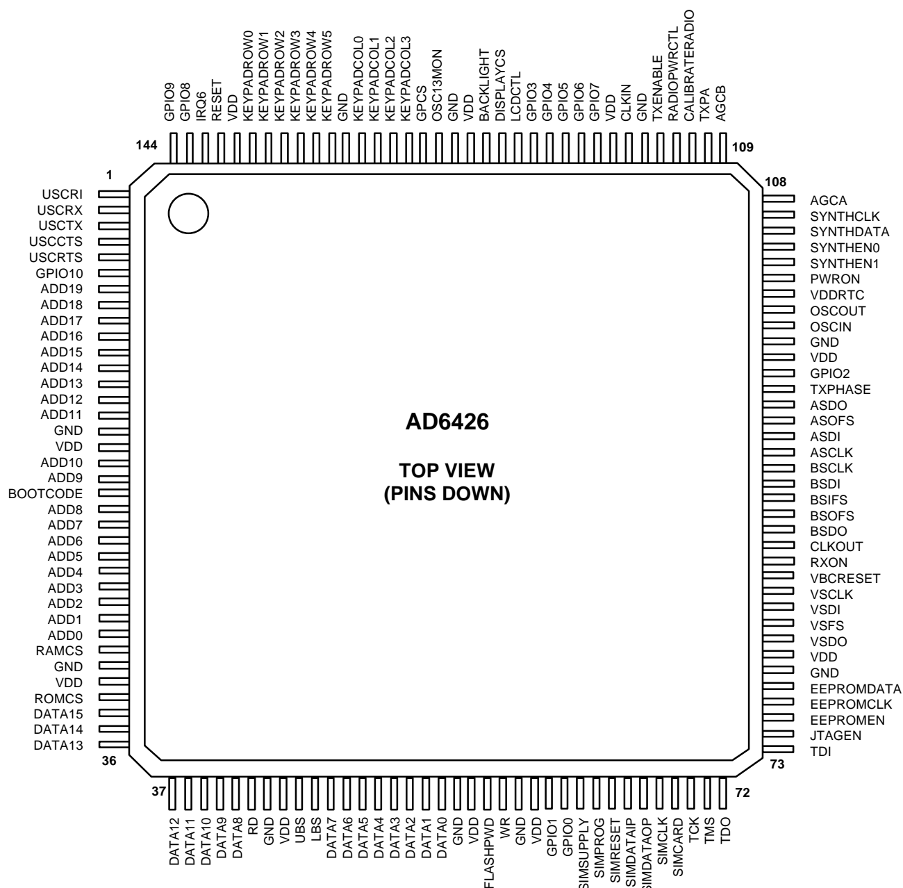
Figure 24: LQFP Pin Locations
