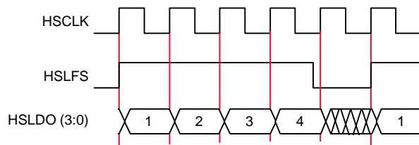
Figure 11. HSL Timing
