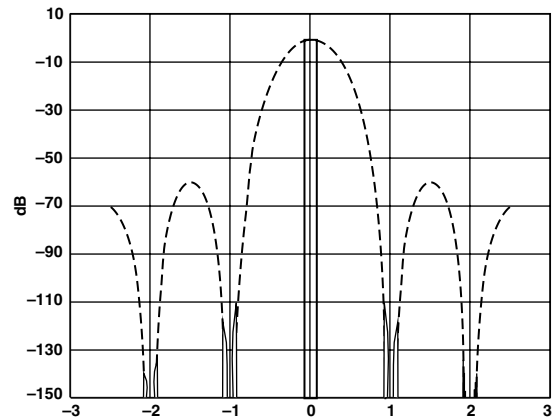
Figure 28. -110 dBc Rejection
