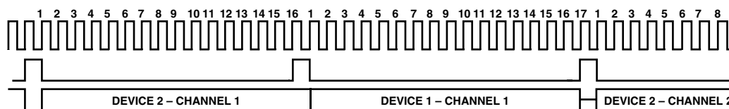
Figure 18. Cascade Timing for a Two-Device Cascade
