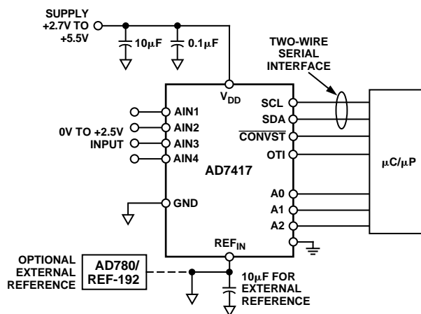
Figure 2. Typical Connection Diagram
