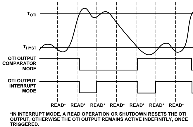
Figure 12. Operation of OTI Output (Shown Active Low)
