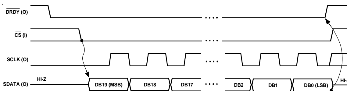
Figure 17. Timing Diagram for the SEC Mode
