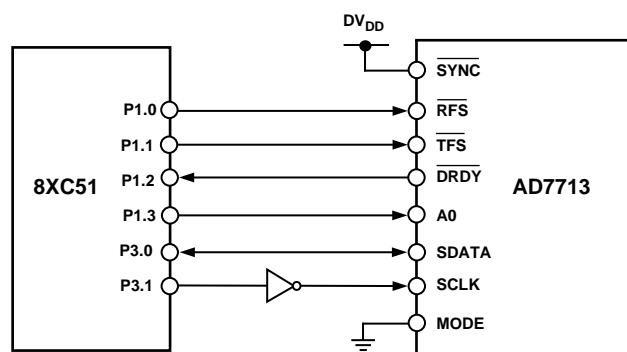
Figure 17. AD7713 to 8XC51 Interface
