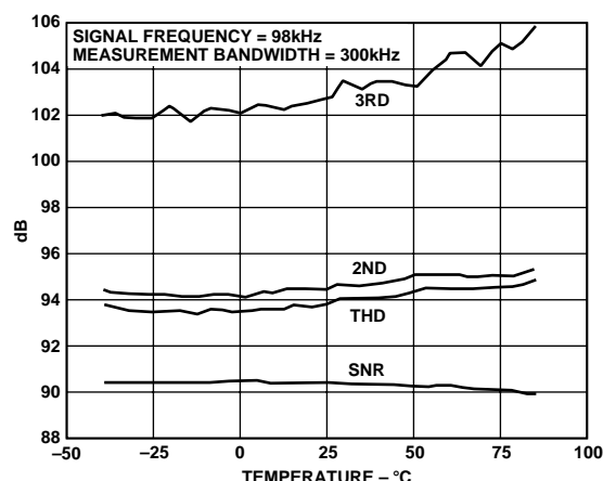
Figure 12. SNR and THD vs. Temperature (Output Data Rate = 600 kHz)
