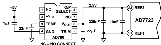
Figure 36. External Reference Circuit Connection
