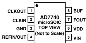
8-Lead microSOIC
