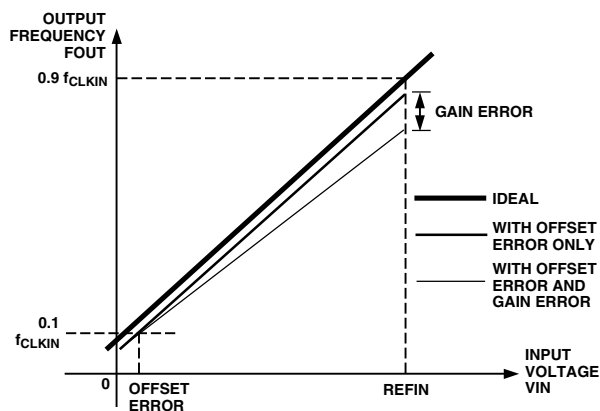
Figure 2. Offset and Gain
