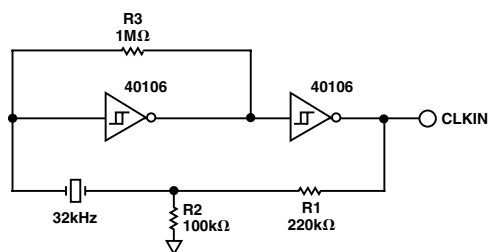
Figure 13. 32 kHz Watch Crystal Circuit
