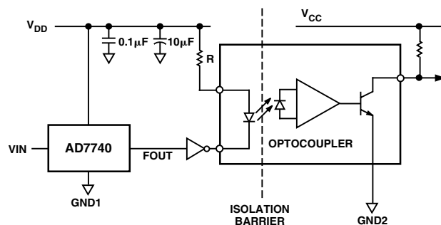
Figure 11. Opto-Isolated Application
