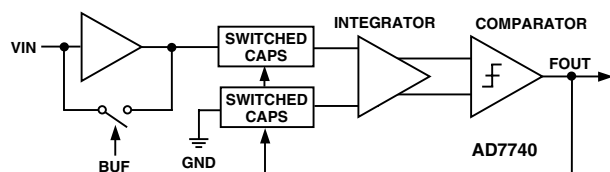
Figure 3. Block Diagram
