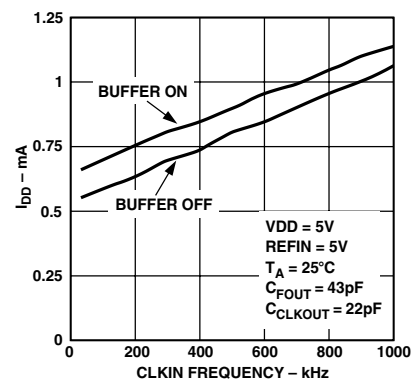
TPC 6. I_{DD} vs. CLKIN (Buffered and Unbuffered)
