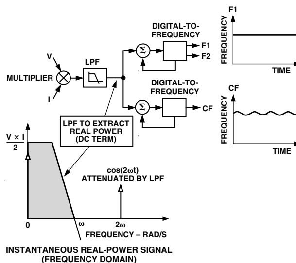
Figure 12. Real-Power-to-Frequency Conversion
