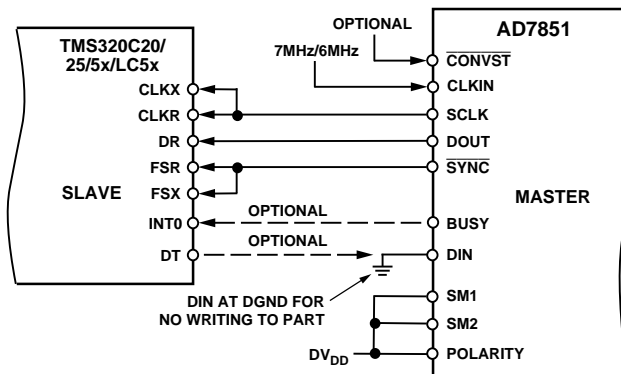
Figure 49. TMS320C20/25/5x Interface
