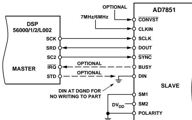
Figure 48. DSP56000/1/2 Interface
