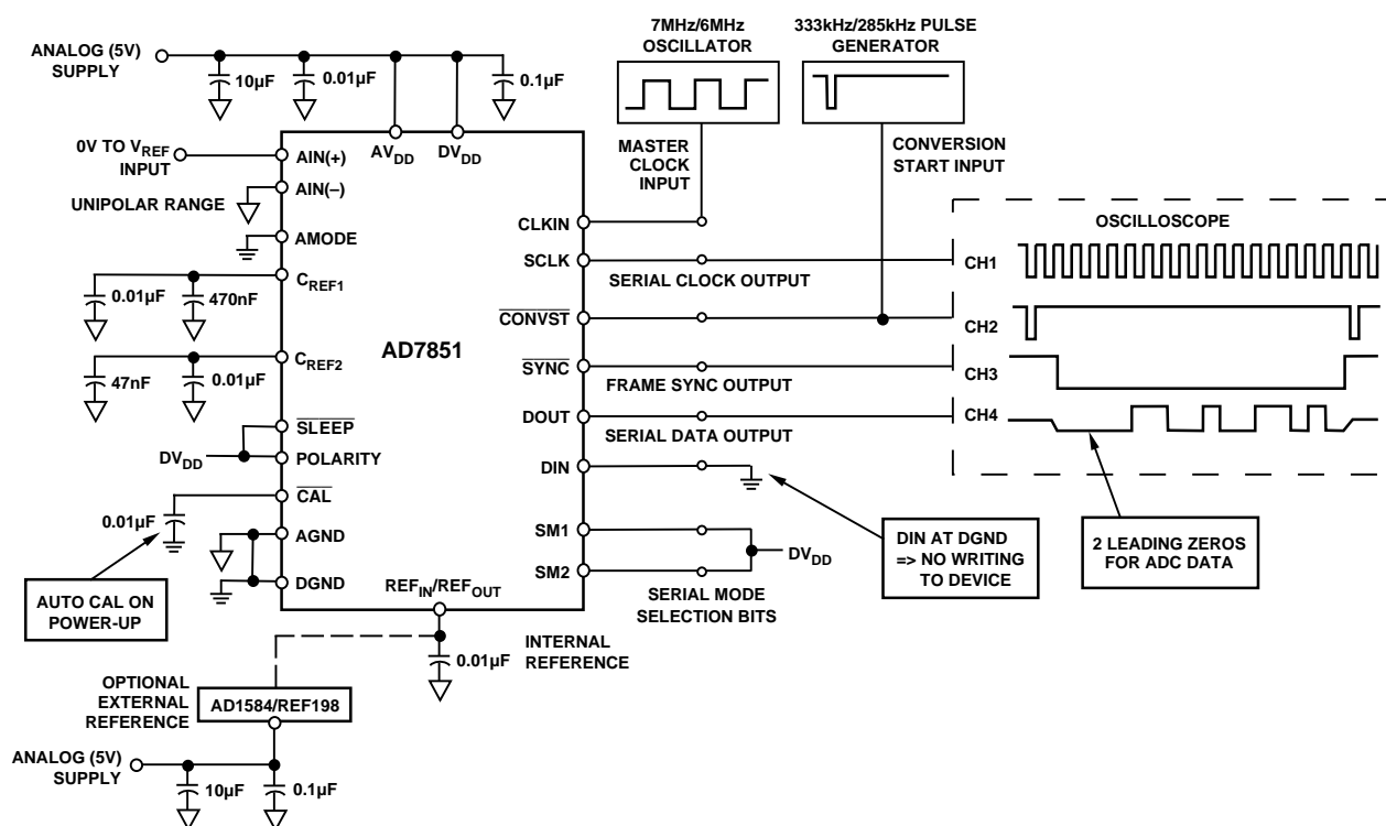
Figure 10. Typical Circuit
