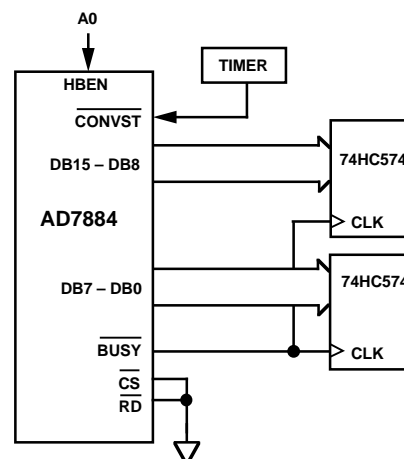
Figure 22. Stand-Alone Operation
