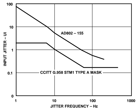
Figure 19. AD802-155 Minimum Acquisition Range vs. Jitter Frequency, T_{MIN} to T_{MAX} V_{MIN} to V_{MAX}
