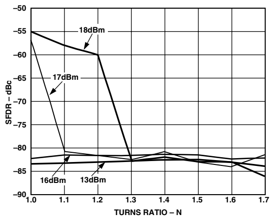
TPC 33. SFDR vs. Turns Ratio; V_S = \pm 12\text{ V} , R_L = 100\ \Omega Line
