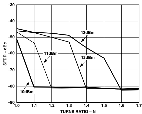
TPC 32. SFDR vs. Turns Ratio; V_S = \pm 6\text{ V} , R_L = 100\ \Omega Line
