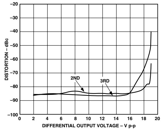
TPC 11. Distortion vs. Output Voltage; f = 100\text{ kHz} , V_S = \pm 6\text{ V} , G = +10 , R_L = 50\ \Omega , Differential
