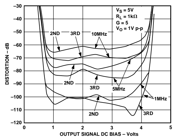
Figure 14. Harmonic Distortion vs. Output Signal DC Bias
