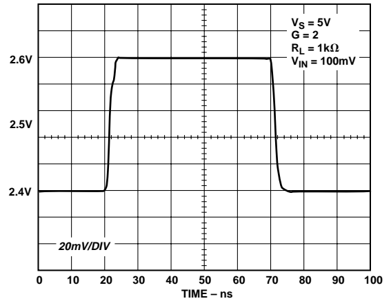
Figure 37. 100 mV Step Response
