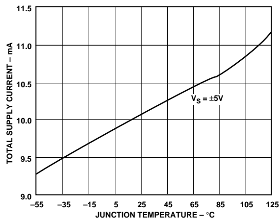
Figure 18. Total Supply Current vs. Temperature
