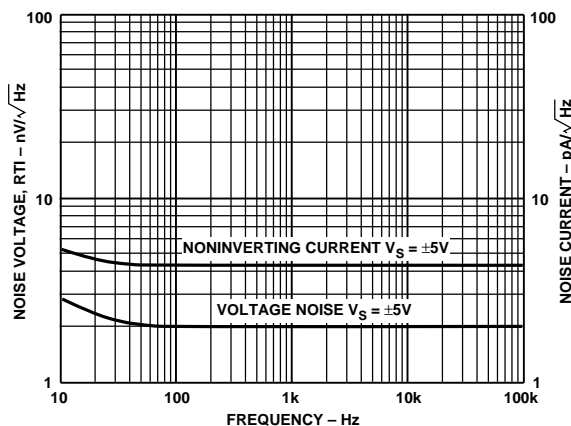
Figure 20. Noise vs. Frequency
