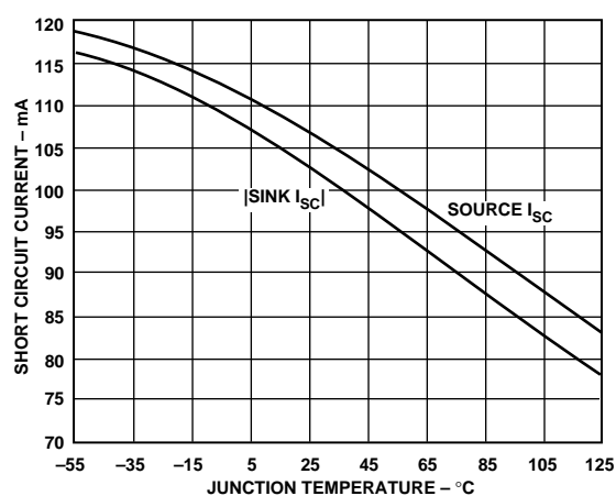
Figure 19. Short Circuit Current vs. Temperature
