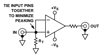
Noninverting Configuration ( G = +1 )
