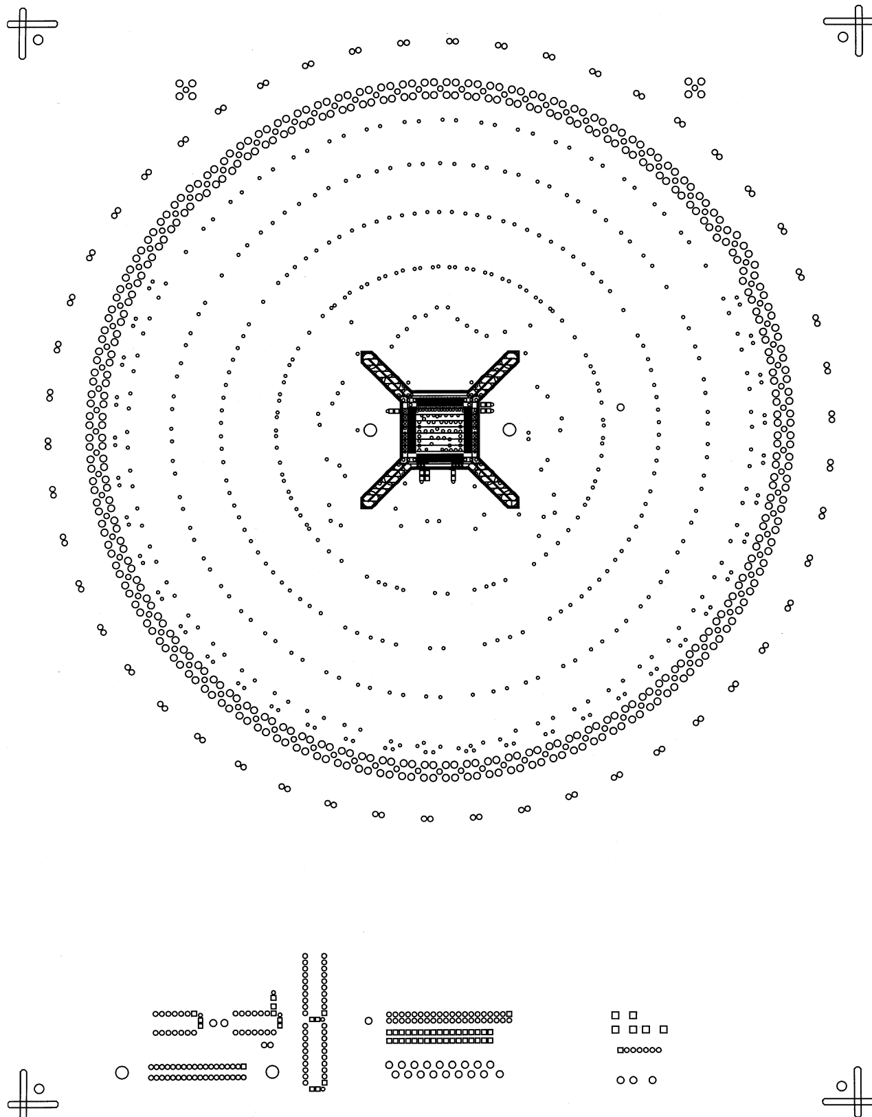
Figure 44. Soldermask Top
