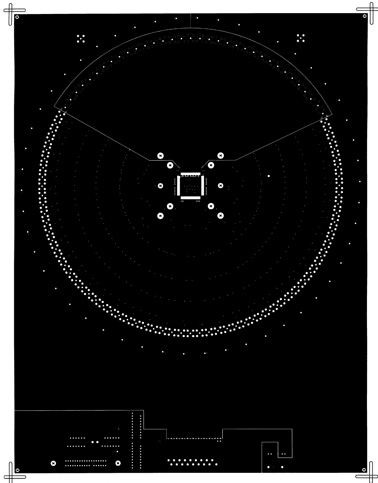
Figure 47. INT1 ( V_{EE} )
