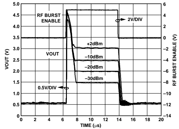
Figure 30. Output Response to RF Burst Input for Various RF Input Levels, Carrier Frequency 900 MHz, CLPF = 0.1 \mu F
