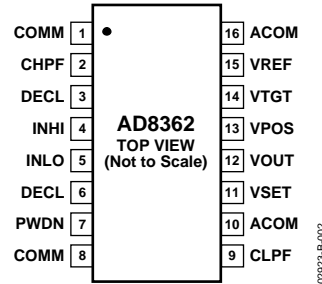
Figure 2. Pin Configuration
