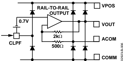
Figure 6. Circuit D
