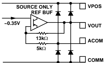
Figure 7. Circuit E
