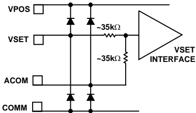
Figure 4. Circuit B
