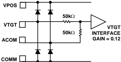
Figure 5. Circuit C
