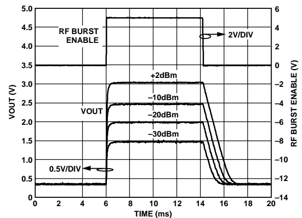
Figure 31. Output Response to RF Burst Input for Various RF Input Levels, Carrier Frequency 900 MHz, CLPF = 0.1 \mu F
