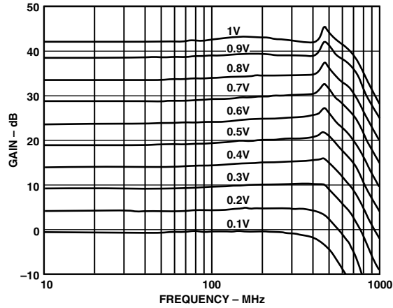
TPC 1. Gain vs. Frequency for Values of V_{\text{GAIN}}
