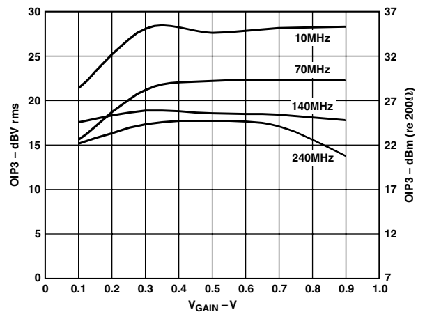
TPC 6. OIP3 vs. V_{\text{GAIN}}
