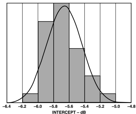
TPC 24. Gain Intercept Distribution at 70 MHz
