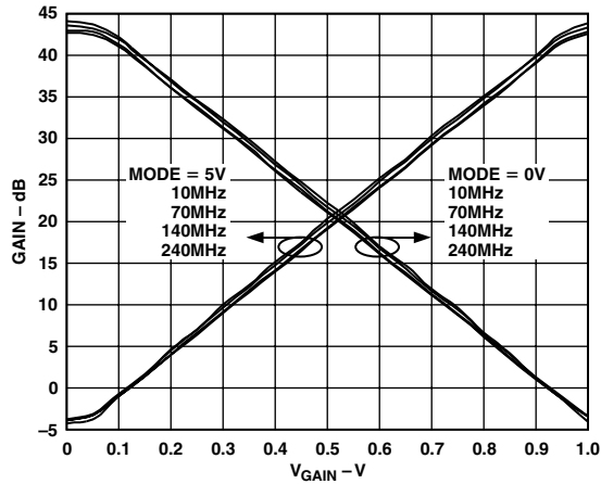
TPC 2. Gain vs. V_{\text{GAIN}} (Mode LO and Mode HI)
