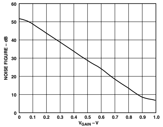
TPC 5. NF (re 200 \Omega ) vs. V_{\text{GAIN}} at 70 MHz
