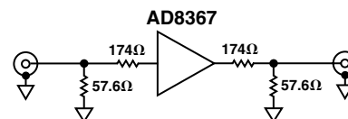
Figure 19. Characterization Test Setup
