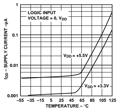
Figure 28. Supply Current vs. Temperature
