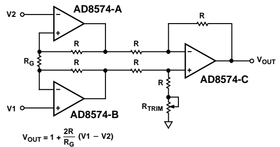
Figure 57. A Discrete Instrumentation Amplifier Configuration
