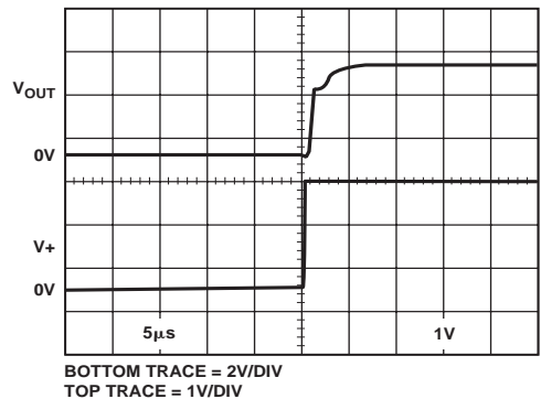
Figure 54a. AD857x Output Behavior on Power-Up
