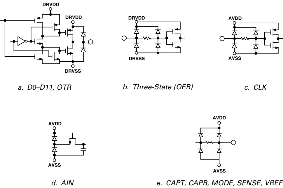
Figure 2. Equivalent Circuits
