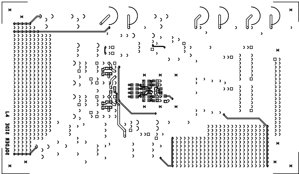
Figure 37. Evaluation Board Solder-Side Layout
