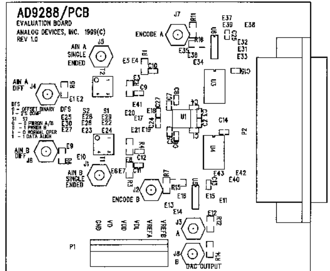
Figure 32. Printed Circuit Board Top Side Silkscreen
