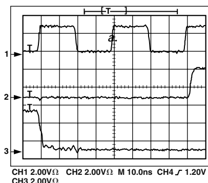
b. Figure 13. RESET Timing of AD9772A with PLL Disabled
