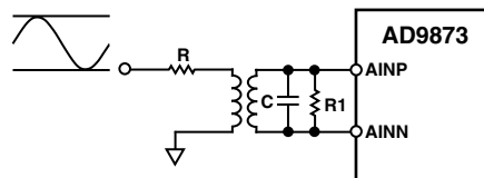
Figure 22. Transformer-Coupled Input
