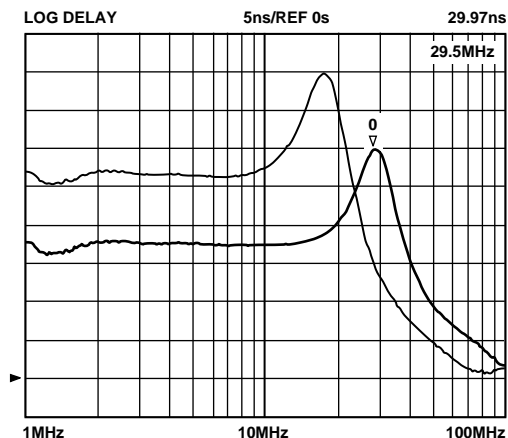
TPC 30. Rx LPF Group Delay, High f_c , 0 x 60 and 0 x 96 Tuning Targets
