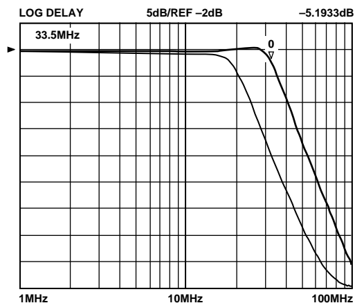
TPC 27. Rx LPF Frequency Response, High f_c , 0 x 60 and 0 x 96 Tuning Targets
