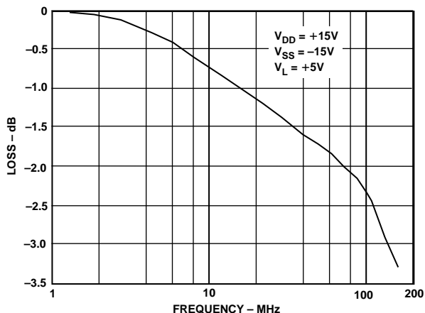
Figure 10. Frequency Response with Switch On
