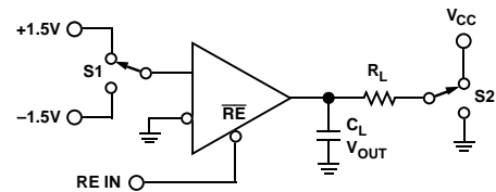
Figure 4. Receiver Enable/Disable Test Circuit
