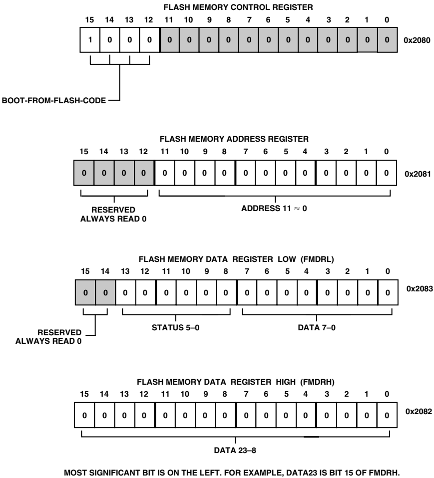
Figure 21. Configuration of Flash Memory Registers
