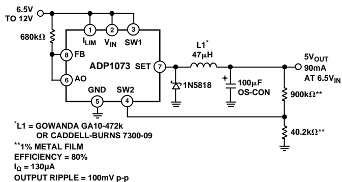
Figure 42. 9 V to 5 V Reduced Noise Step-Down Converter
