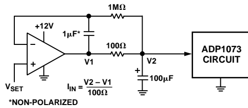
Figure 24. Test Circuit Measures No Load Quiescent Current of ADP1073 Converter
