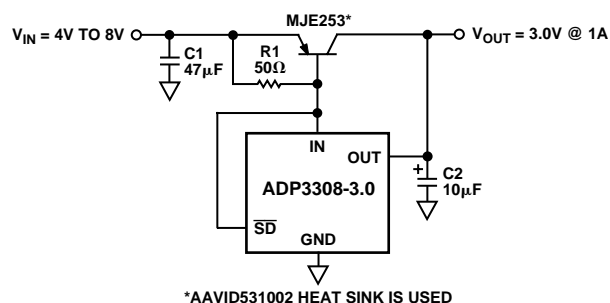
Figure 22. Higher Output Current Linear Regulator
