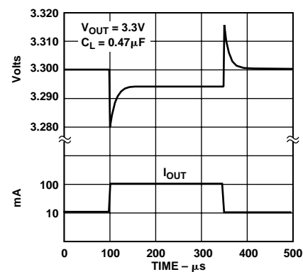
Figure 13. Load Transient
