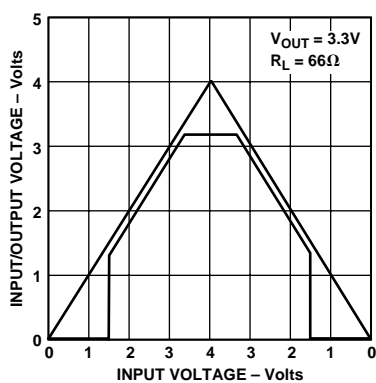
Figure 9. Power-Up/Power-Down
