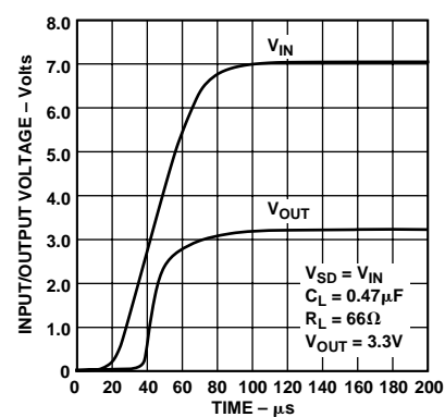
Figure 10. Power-Up Overshoot
