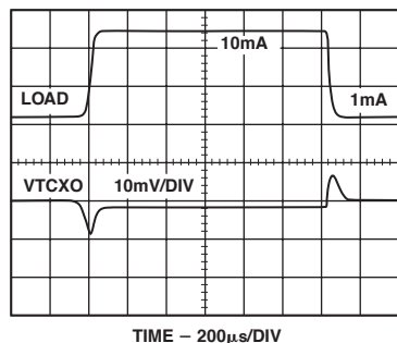
TPC 10. VTCXO Load Step
