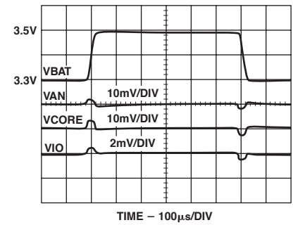
TPC 9. Line Transient Response, Maximum Loads
