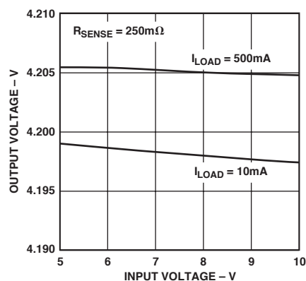
TPC 21. Charger V_{OUT} vs. V_{IN}
