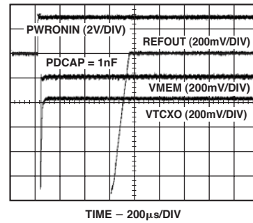
TPC 18. Turn On Transient by PWRONIN, Maximum Load
