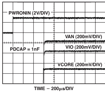
TPC 17. Turn On Transient by PWRONIN, Maximum Load
