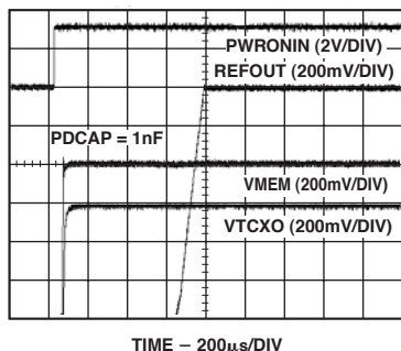
TPC 16. Turn On Transient by PWRONIN, Minimum Load
