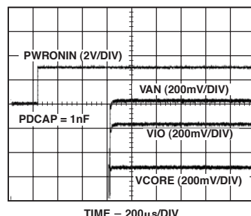
TPC 15. Turn On Transient by PWRONIN, Minimum Load
