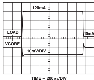
TPC 13. VCORE Load Step
