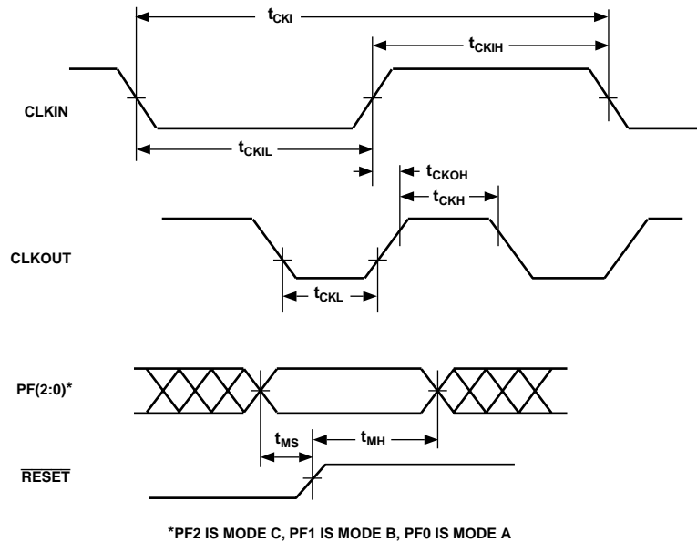
Figure 8. Clock Signals
