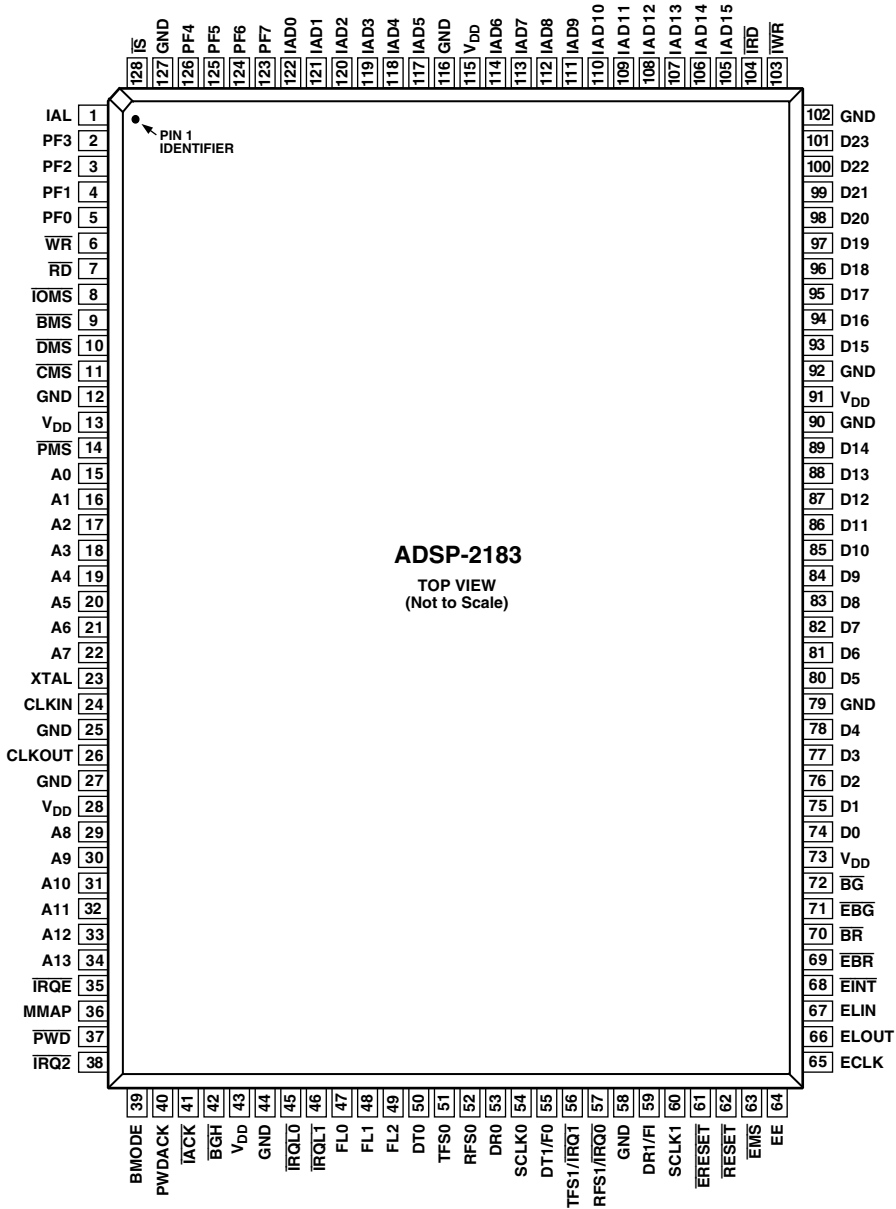
128-Lead LQFP Package Pinout
