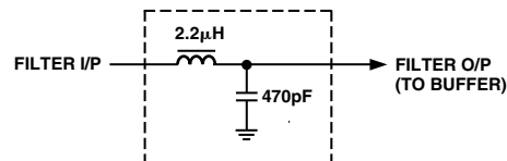
Figure 102. Output Filter for 4× Oversampling Mode
