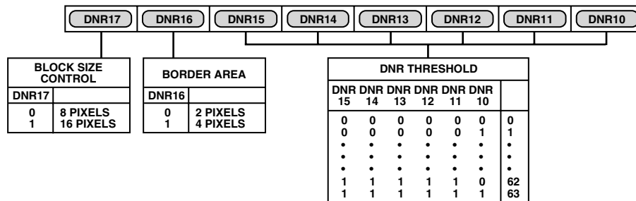
Figure 86. DNR Register 1
