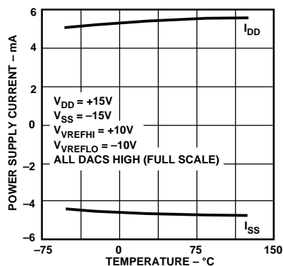
Figure 23. Power Supply Current vs. Temperature
