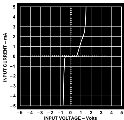
Figure 43. Input Overvoltage I-V Characteristics of the OP284
