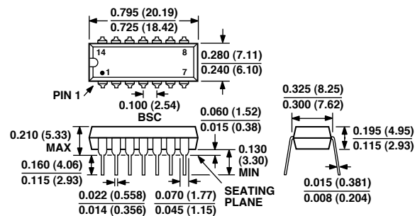
14-Lead PDIP Package (N-14)
