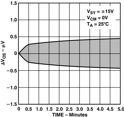
Figure 41. Warm-Up Drift
