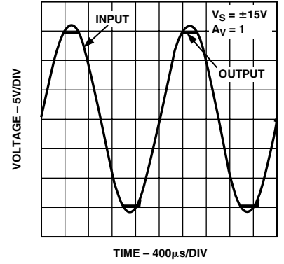
Figure 24. No Phase Reversal
