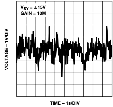
Figure 30. 0.1 Hz to 10 Hz Input Voltage Noise
