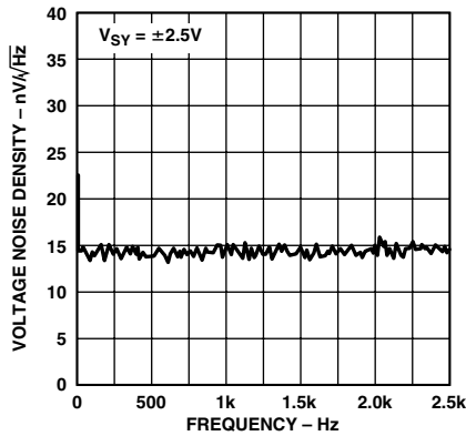
Figure 34. Voltage Noise Density
