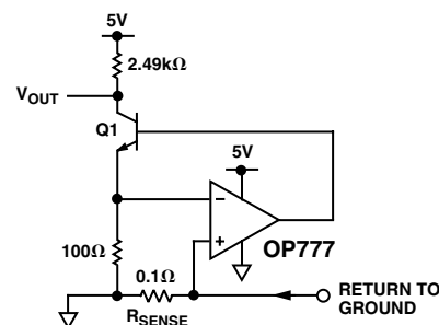
Figure 48. A Low-Side Load Current Monitor
