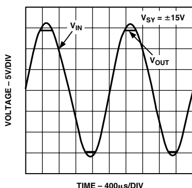
Figure 45. No Phase Reversal
