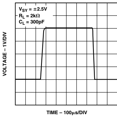
Figure 16. Large Signal Transient Response
