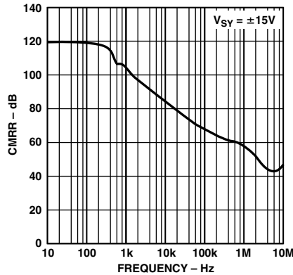
Figure 26. CMRR vs. Frequency
