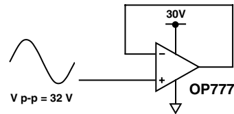
Figure 44a. Unity Gain Follower
