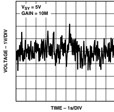
Figure 29. 0.1 Hz to 10 Hz Input Voltage Noise
