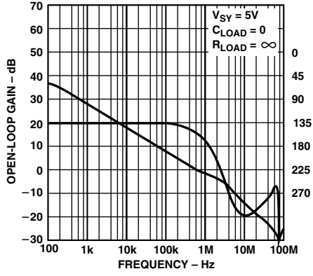
Figure 11. Open Loop Gain and Phase Shift vs. Frequency
