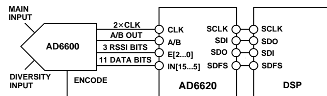
Figure 61. Implementation of a Narrow Band Receiver
