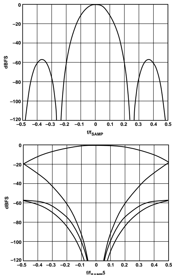
Figure 43. CIC5 Alias Rejection, M_{\text{CIC5}} = 4
