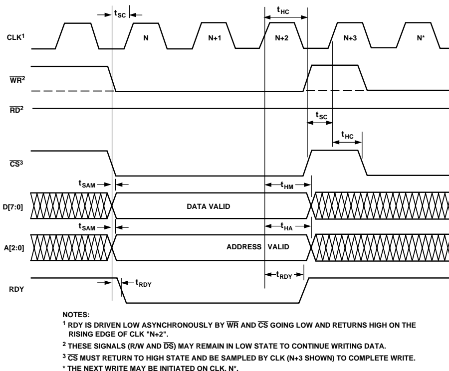
Figure 49. Mode 0 Write (MODE = GND)
