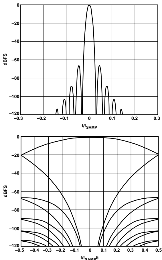
Figure 44. CIC5 Alias Rejection, M_{\text{CIC5}} = 32
