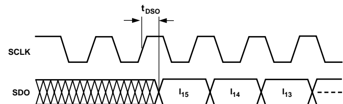
Figure 12. Serial Output Data Switching Characteristics
