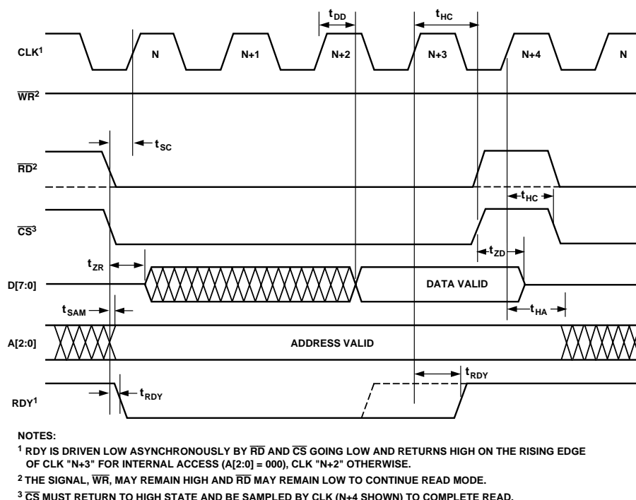
Figure 48. Mode 0 Read (MODE = GND)
