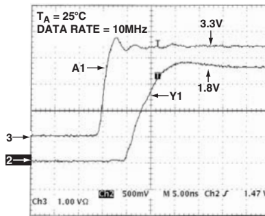
TPC 14. Input/Output V_{CC1} = 3.3V, V_{CC2} = 1.8V
