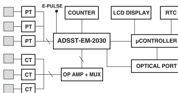
POLY PHASE ENERGY METER USING THE ADSST-EM-2030
