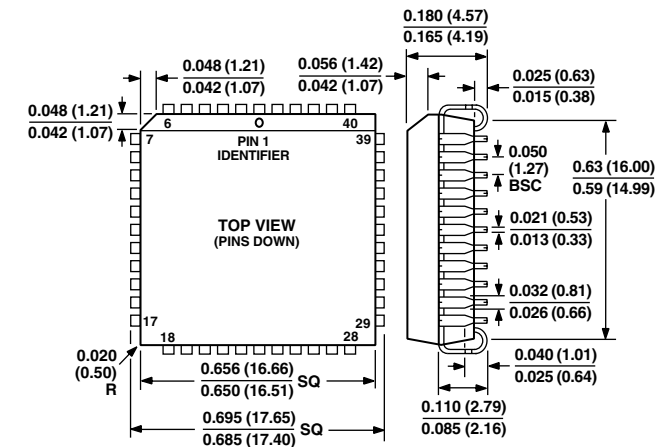
44-Lead PLCC (P-44A)
