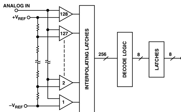
Figure 1. AD9058 Comparator Block Diagram
