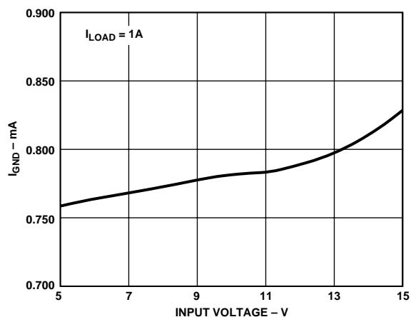
Figure 6. I_{GND} vs. V_{IN} ( I_{LOAD} = 1 A )*
