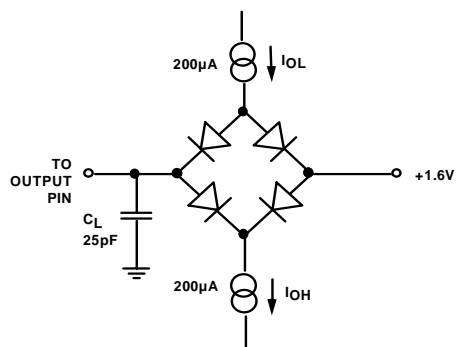
Figure 1. Load Circuit for Digital Output Timing Specifications
