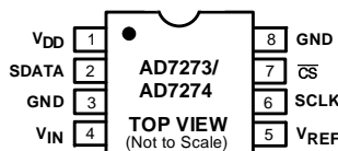
8-lead TSOT
