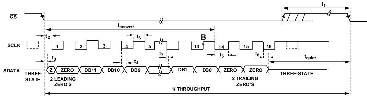
Figure 5. AD7274 Serial Interface Timing Diagram
