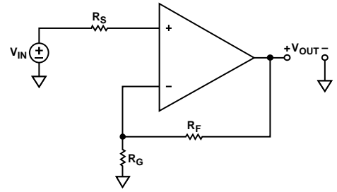
Figure 64. Noninverting Configuration
